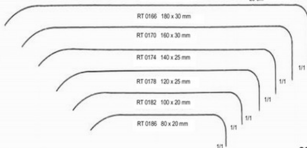
BRUNNER RT 0166 - RT 0186 25 cm
